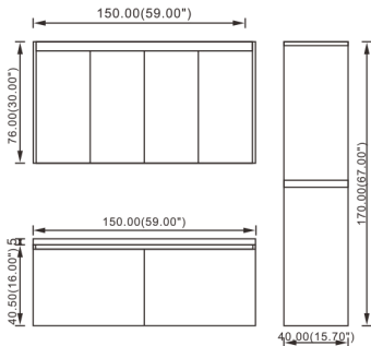
60" AVANTI Medicine Cabinet SKU# AV-760
