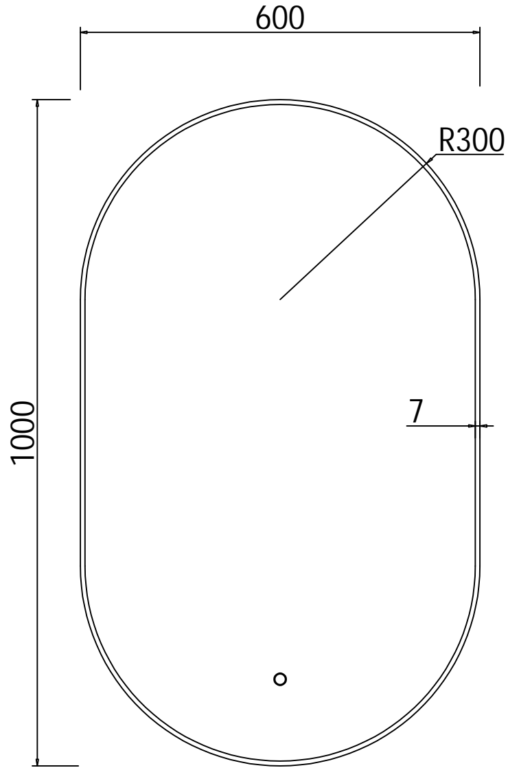
front view
