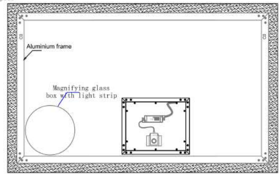
Back View
