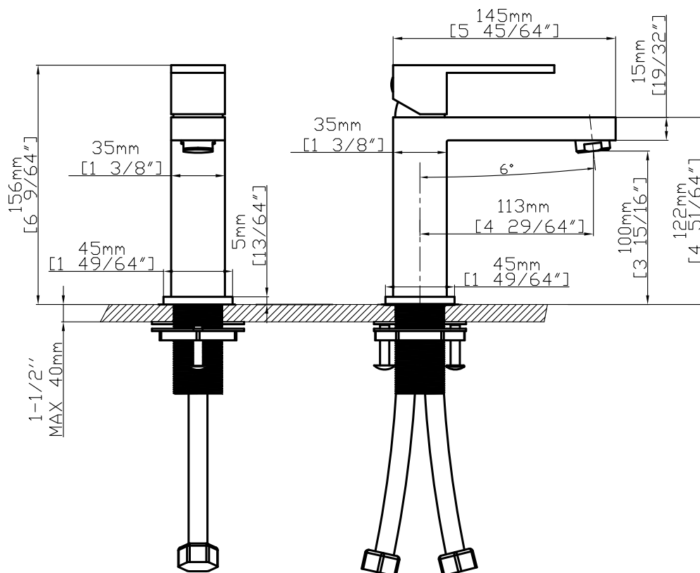
CRITICAL DIMENSIONS
