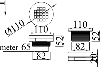
Drain
