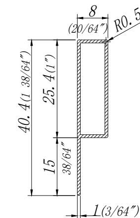
Movable flange
