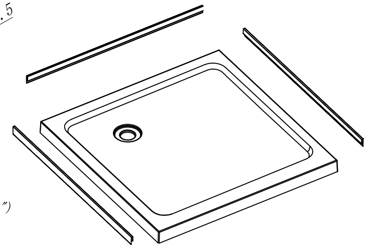
Movable flange
