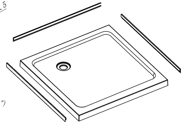
Movable flange
