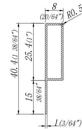
Movable flange
