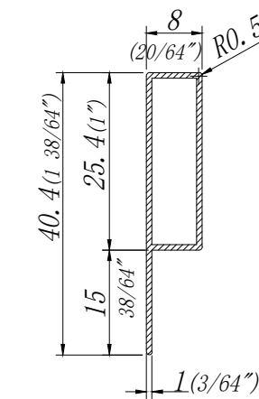
Movable flange
