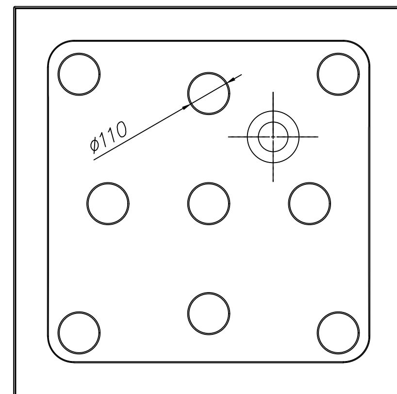
Bottom view
