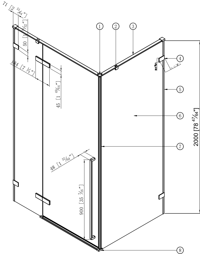
Front view
